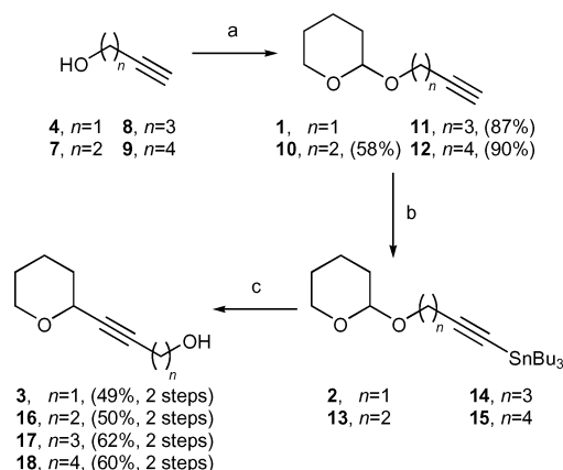
Scheme 5 Reagents and conditions: [a]. DHP, CSA, CH 2 Cl 2 , 0 °C; [b]. n -BuLi, THF, -78 °C, then Bu 3 SnCl, THF; [c] BF 3 ·OEt 2 , CH 2 Cl 2 , -10 °C. DHP = 3,4-dihydropyran, CSA = camphorsulfonic acid.
