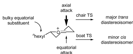
Fig. 1 Diastereoselective rearrangement of disubstituted pyrans.
