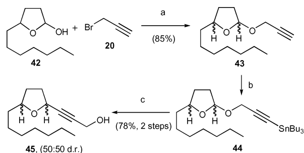
Scheme 9 Reagents and conditions: [a]. KHMDS, THF, -78^{\circ}\text{C} (85%); [b]. n -BuLi, THF, -78^{\circ}\text{C} , then \text{Bu}_3\text{SnCl} , THF; [c] \text{BF}_3\cdot\text{OEt}_2 , \text{CH}_2\text{Cl}_2 , -10^{\circ}\text{C} (78%, 2 steps). KHMDS = potassium hexamethyldisilazide.
