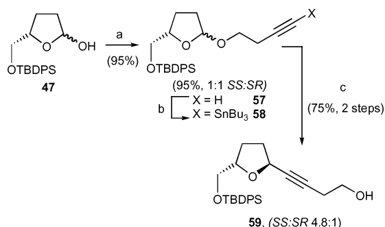
Scheme 13 Reagents and conditions: [a]. but-3-yn-1-ol, Amberlyst A-15 ® , benzene, 15 min, reflux, (95%); [b]. n -BuLi, THF, 30 min, -78\text{ }^{\circ}\text{C} ; \text{Bu}_3\text{SnCl} , 30 min, -78\text{ }^{\circ}\text{C} \rightarrow \text{rt} ; [c]. \text{BF}_3 \cdot \text{OEt}_2 , \text{CH}_2\text{Cl}_2 , 5 min, -10\text{ }^{\circ}\text{C} , (75%, 2 steps, 4.8 : 1). TBDPS = tert -butyldiphenylsilyl.
