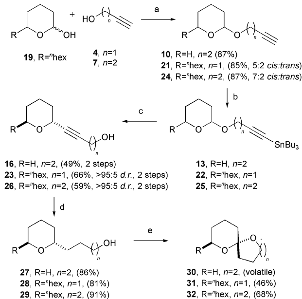
Scheme 7 Reagents and conditions: [a]. Amberlyst® A-15, toluene, reflux; [b]. n -BuLi, THF, -78^{\circ}\text{C} , then \text{Bu}_3\text{SnCl} , THF; [c] \text{BF}_3\cdot\text{OEt}_2 , \text{CH}_2\text{Cl}_2 , -10^{\circ}\text{C} ; [d]. Raney nickel, \text{H}_2 , EtOH, rt; [e]. \text{I}_2 , \text{HgO} , cyclohexane, reflux.
