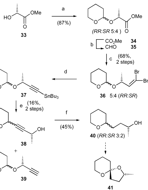
Scheme 8 Reagents and conditions: [a]. DHP, CSA, 0^{\circ}\text{C} , (87%, 5 : 4 d.r.); [b]. DIBAL-H, \text{Et}_2\text{O} , -78^{\circ}\text{C} ; [c]. \text{PPh}_3 , \text{CBr}_4 , \text{CH}_2\text{Cl}_2 , (68%, 2 steps, 5 : 4 d.r.); [d]. n -BuLi, THF, -78^{\circ}\text{C} , then \text{Bu}_3\text{SnCl} , THF; [e]. \text{BF}_3\cdot\text{OEt}_2 , \text{CH}_2\text{Cl}_2 , -10^{\circ}\text{C} , (16%, 3 steps); [f]. Raney nickel, \text{H}_2 , EtOH, rt, (45%, 3 : 2 d.r.). DHP = 3,4-dihydropyran, DIBAL-H = diisobutylaluminium hydride.
